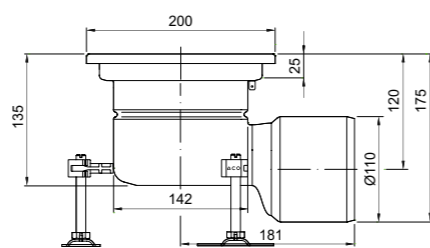
EG Compact 200x200mm DN110 Salida Horizontal Saída Horizontal
