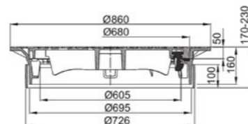
Tapa CityTop Tampa CityTop BITUPLAN P Fix 160
