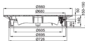
Tapa CityTop Tampa CityTop BITUPLAN P Fix 140
