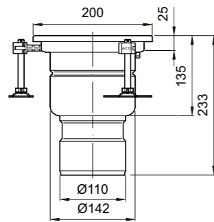
EG Compact 200x200mm DN110 Salida Vertical Saída Vertical
