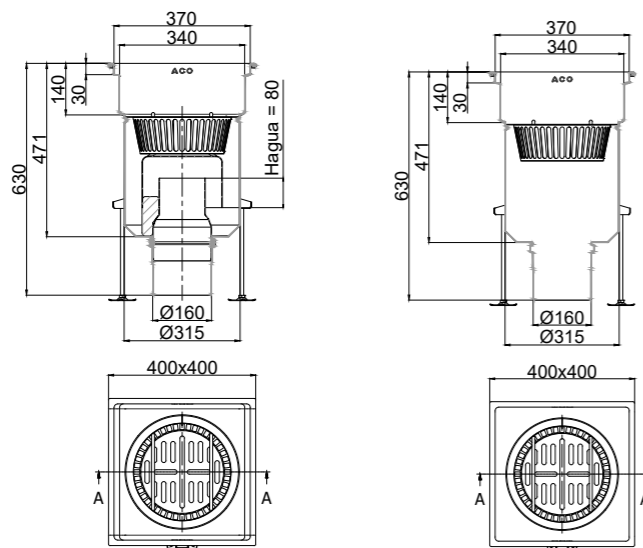
EG400 400x400mm DN160 Salida Vertical Saída Vertical
