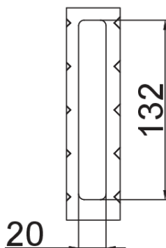
Detalle A (2:1)
