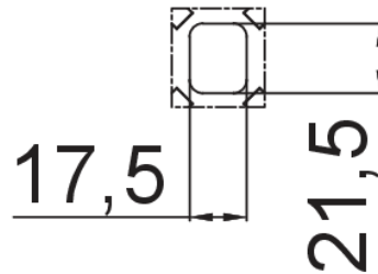
Detalle A (2:1)
