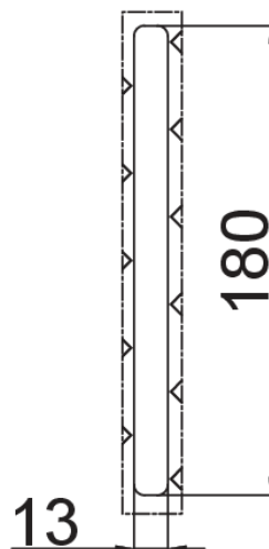
Detalle A (2:1)
