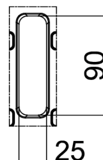
Detalle A (2:1)
